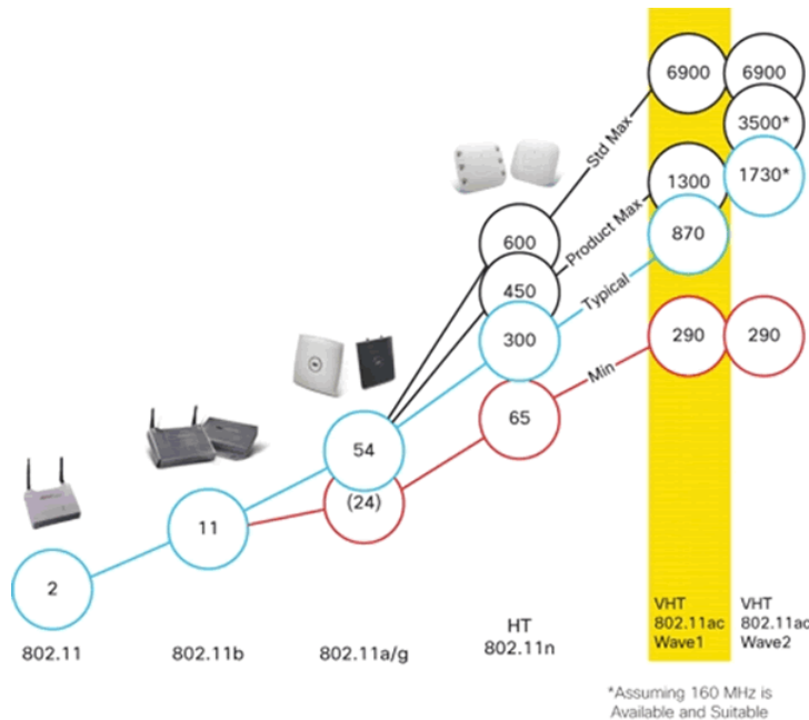
Figure 1: Evolution of 802.11. Values in the circles represent throughput in megabits per second (Mbps). (Source: Cisco)
